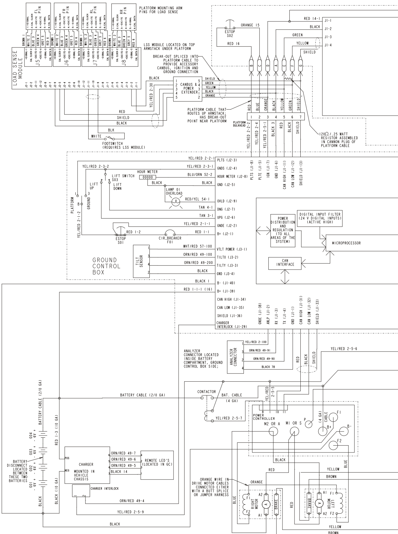
FIGURE 7-2. ELECTRICAL SCHEMATIC (FOR S/N USAGE SEE CHART)
