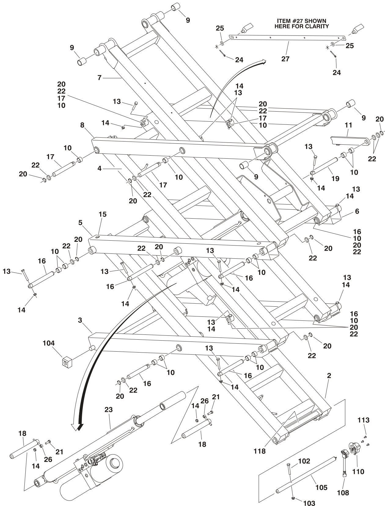
FIGURE 3-2.SCISSOR ARMS INSTALLATION - 1930ES (USA BUILT MACHINES S/N 0200150266 TO S/N 0200152825 & BELGIUM BUILT MACHINES S/N 1200007882 TO S/N 1200008481)
