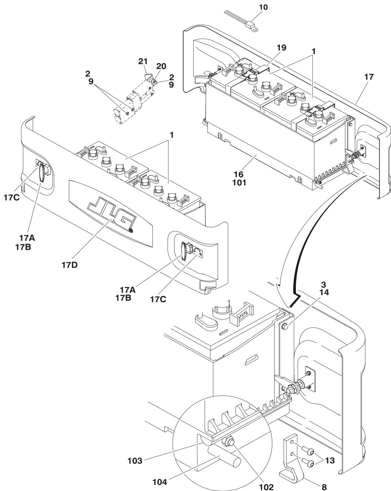
FIGURE 2-1.BATTERIES AND COVERS INSTALLATION
