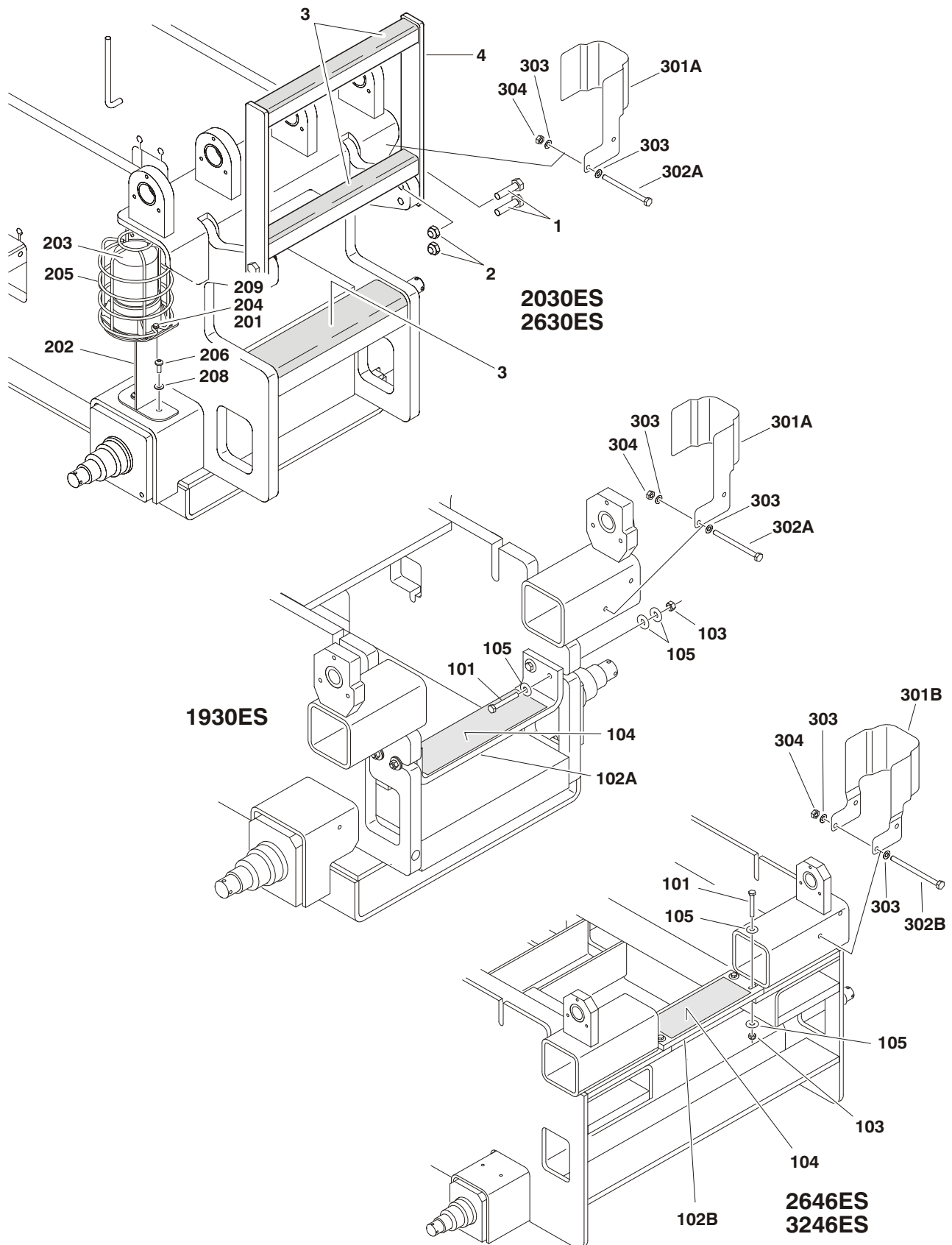
FIGURE 1-10. LADDERS, BEACON LIGHT & ROTARY SENSOR COVER INSTALLATION
