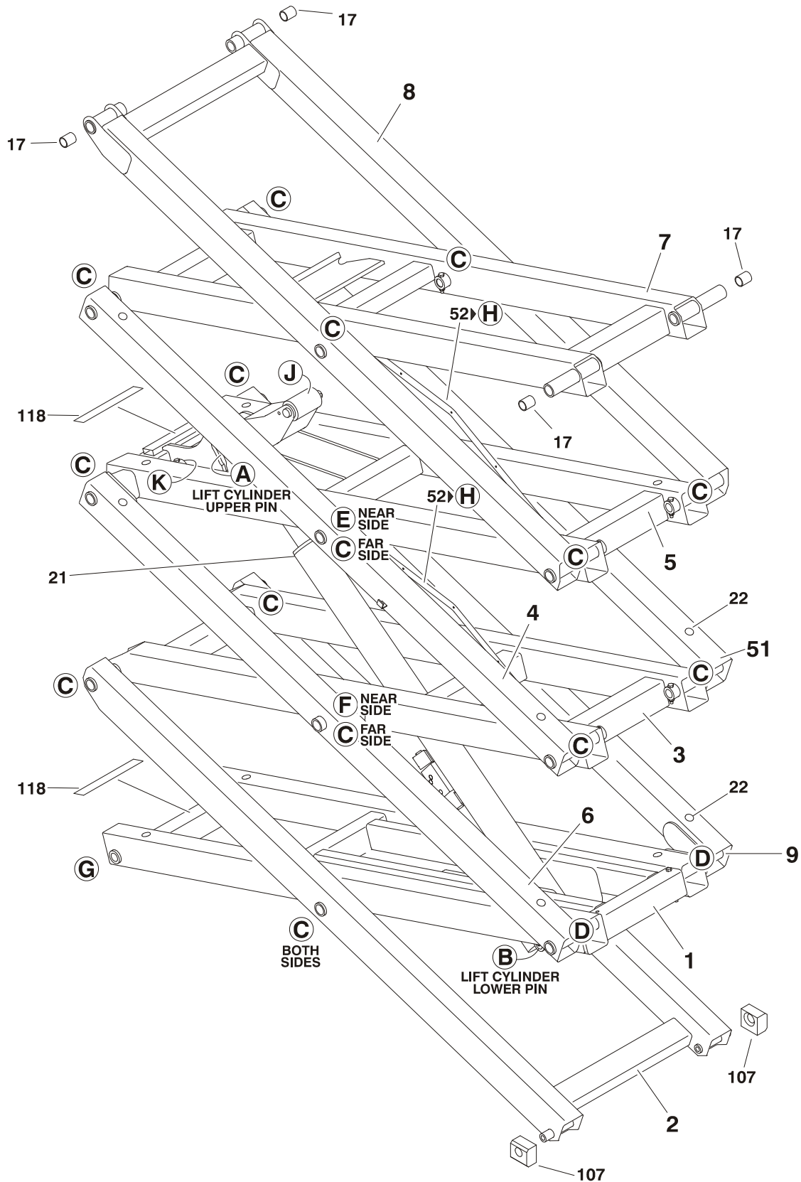
FIGURE 3-6.SCISSOR ARMS INSTALLATION - 2646ES/3246ES (USA BUILT MACHINES S/N 0200151606 TO S/N 0200152825 & BELGIUM BUILT MACHINES BUILT S/N 1200008265 TO S/N 1200008481)
