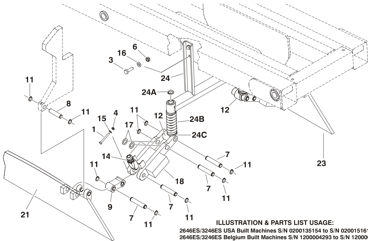
FIGURE 1-6. POTHOLE PROTECTION INSTALLATION (2646ES/3246ES)
