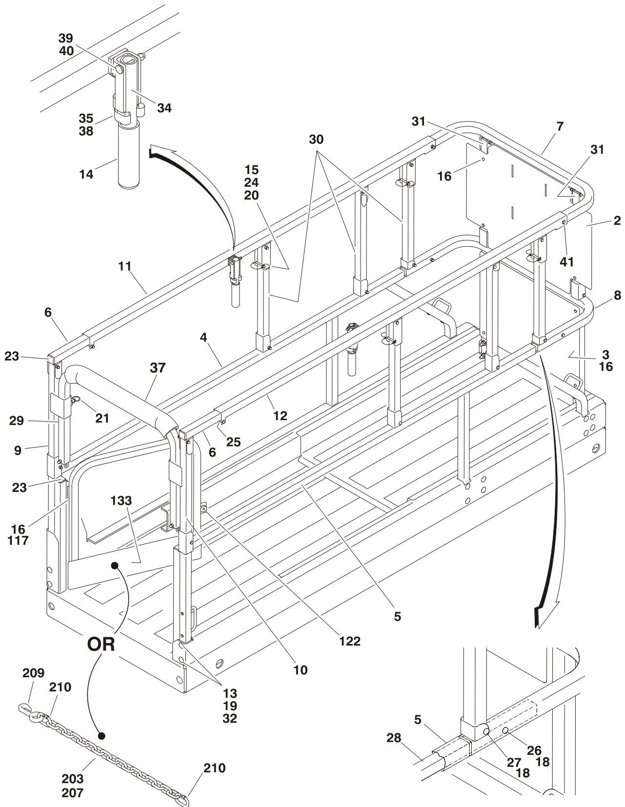
FIGURE 4-6.RAIL INSTALLATION - 2030ES/2630ES
