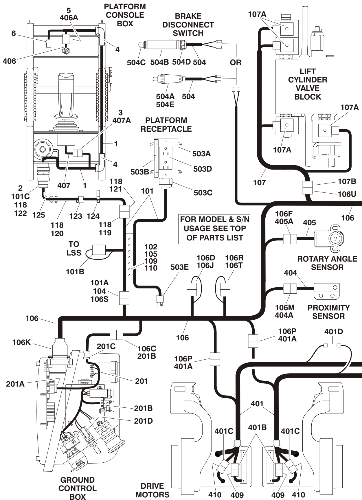
FIGURE 7-3. ELECTRICAL COMPONENTS INSTALLATION (FOR MODEL & S/N USAGE SEE TOP OF PARTS LIST)
