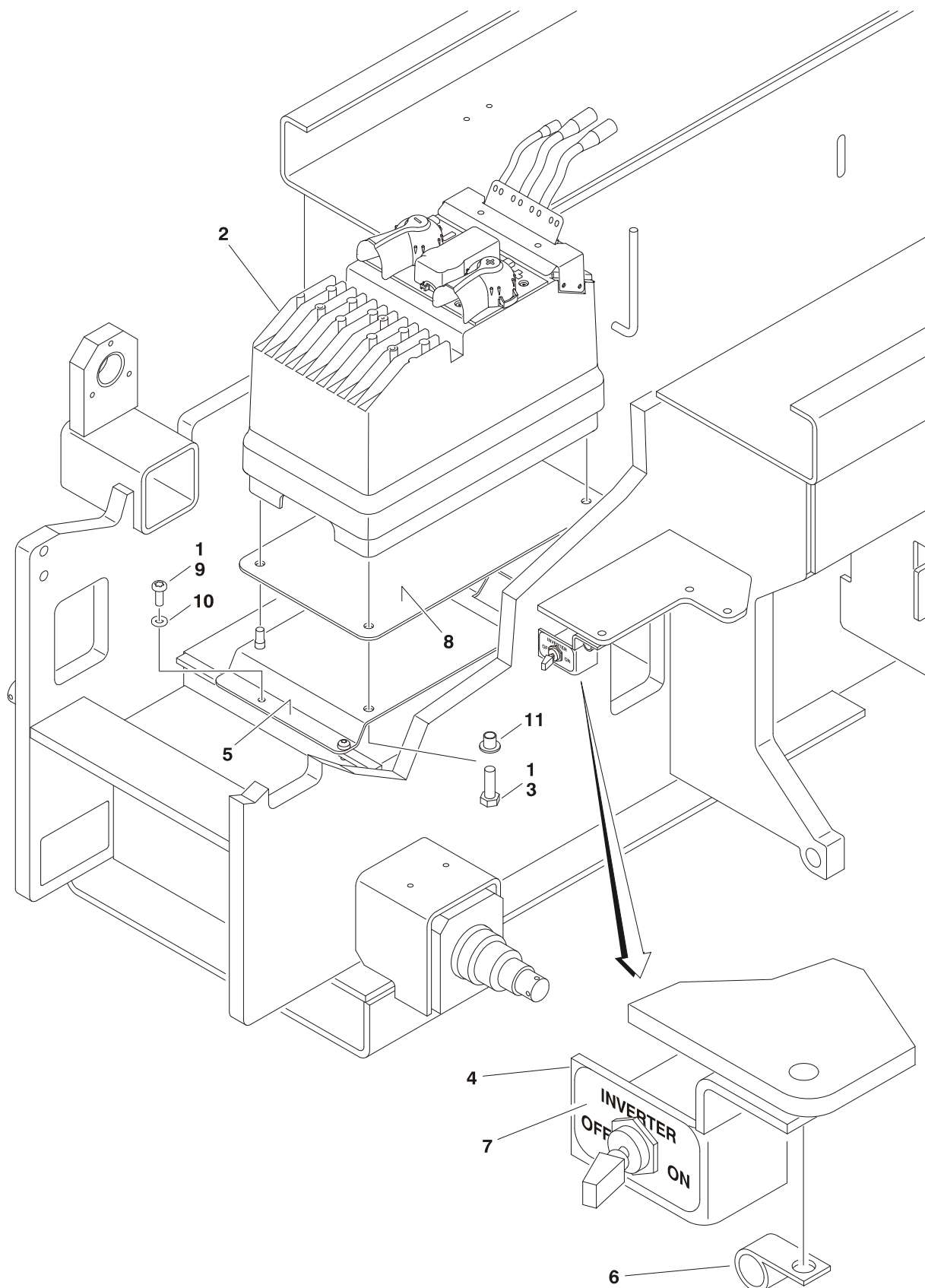
FIGURE 1-9. BATTERY CHARGER WITH INVERTER ASSEMBLY AND INSTALLATION (OPTIONAL ON ANSI SPEC MACHINES)
