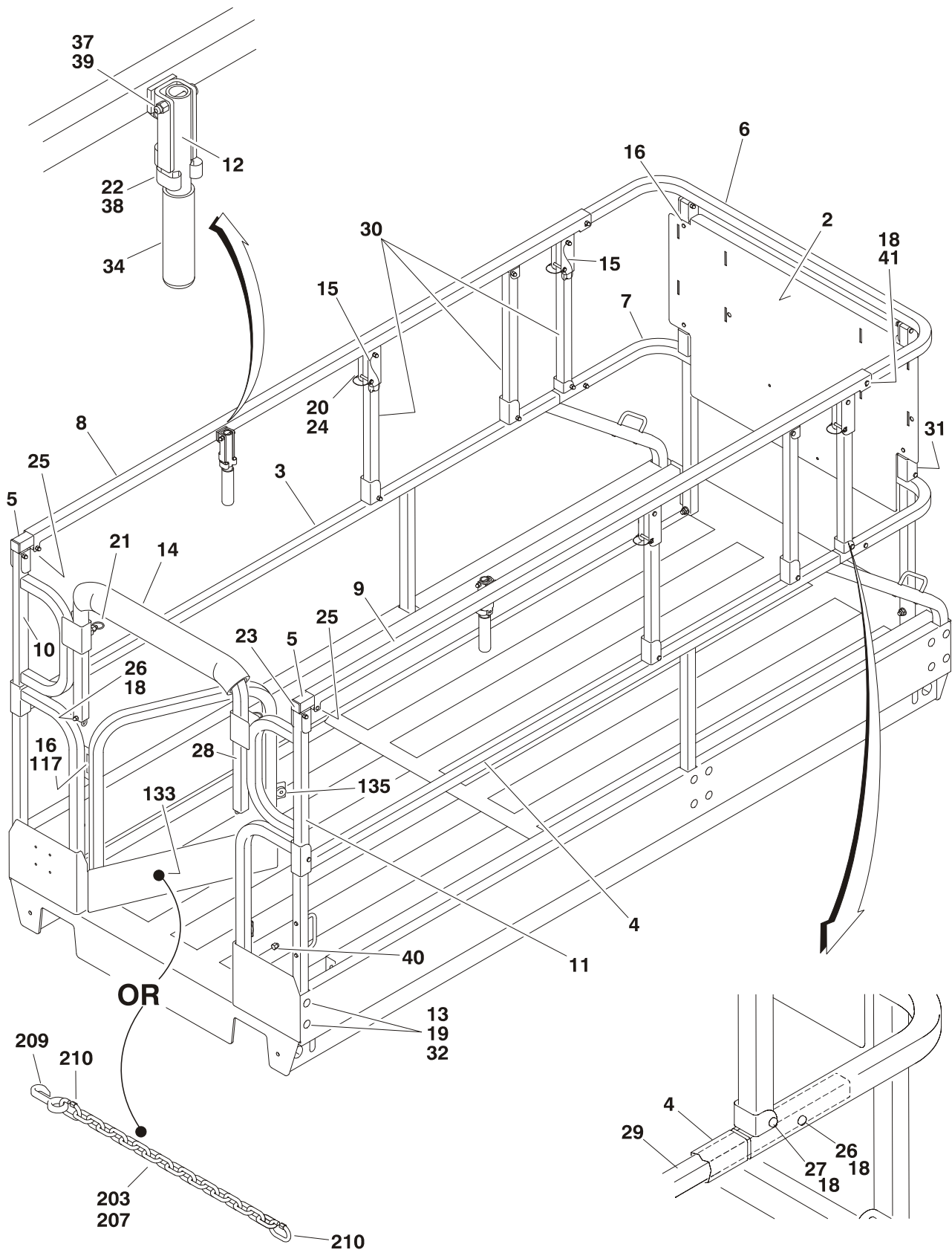
FIGURE 4-7. RAIL INSTALLATION - 2646ES/3246ES (USA BUILT MACHINES S/N 0200135154 TO S/N 0200151585 & BELGIUM BUILT MACHINES S/N 1200004293 TO S/N 1200008265)
