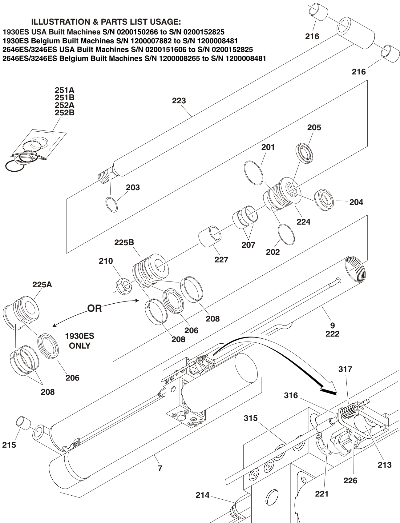
FIGURE 5-2. LIFT CYLINDER ASSEMBLY (FOR MODEL & S/N USAGE SEE TOP OF PARTS LISTS)
