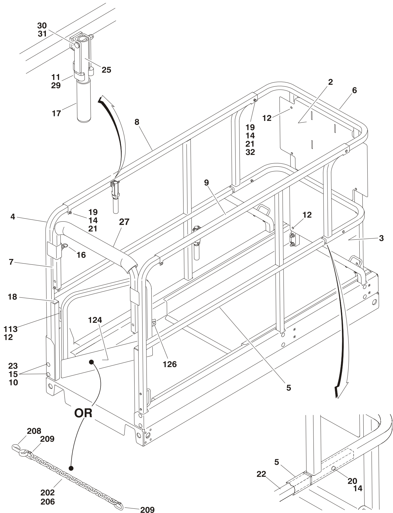
FIGURE 4-2.RAIL (FIXED) INSTALLATION - 1930ES (USA BUILT MACHINES S/N 0200135154 TO S/N 0200150266 & BELGIUM BUILT MACHINES S/N 1200004293 TO S/N 1200007882)
