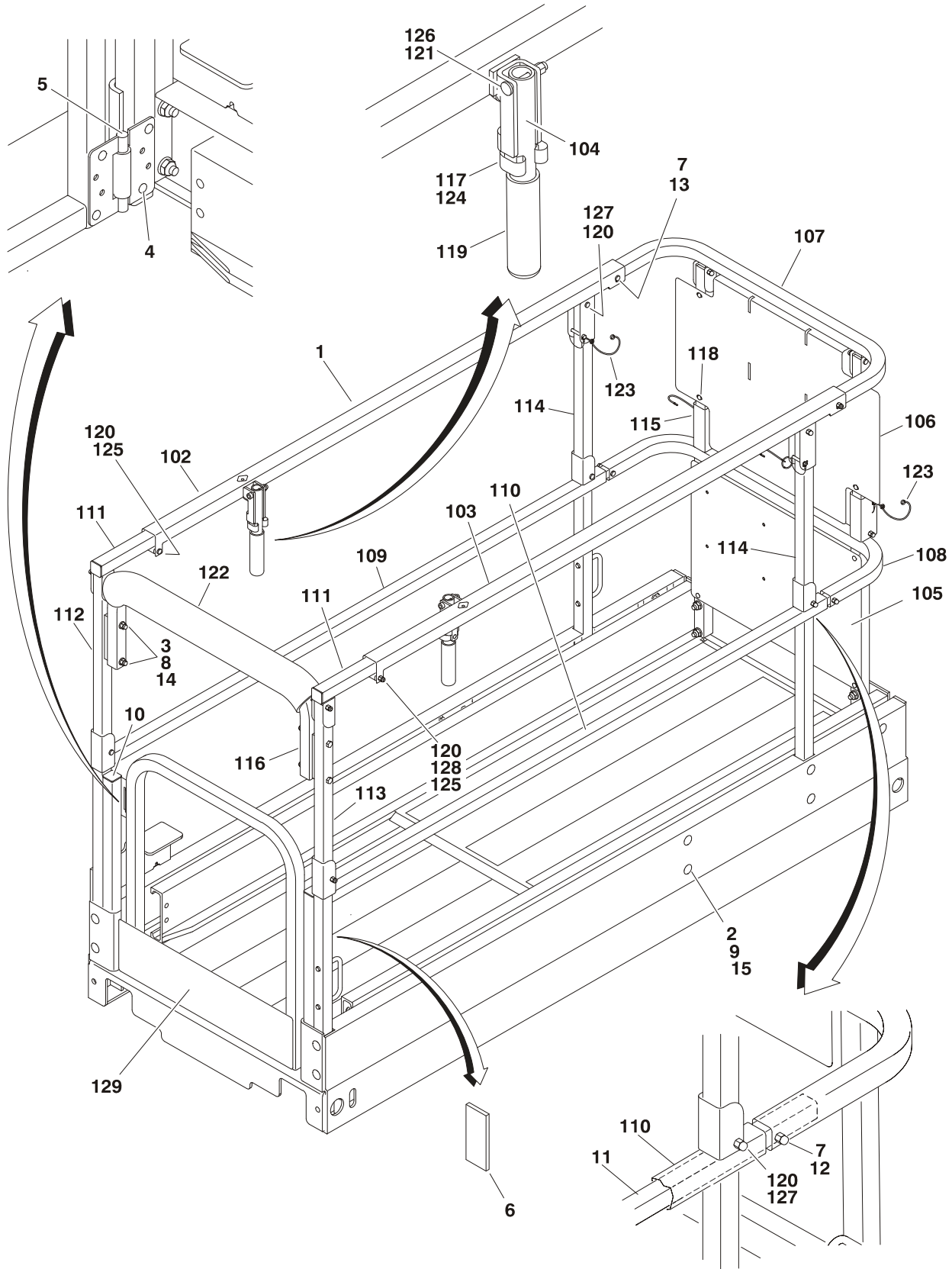
FIGURE 4-5.RAIL (FOLD-DOWN) INSTALLATION - 1930ES (USA BUILT MACHINES S/N 0200150266 TO S/N 0200152825 & BELGIUM BUILT MACHINES S/N 1200007882 TO S/N 1200008481)
