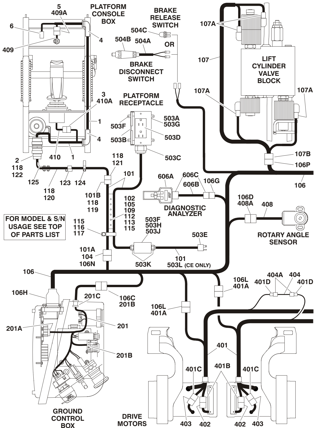
FIGURE 7-4. ELECTRICAL COMPONENTS INSTALLATION (FOR MODEL & S/N USAGE SEE TOP OF PARTS LIST)
