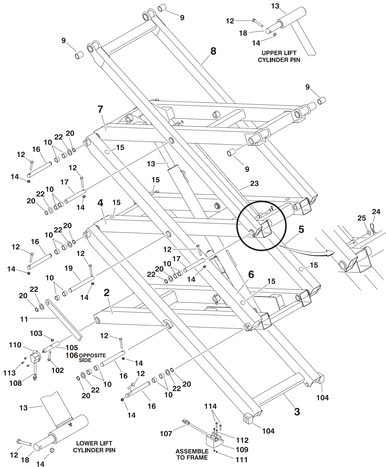
FIGURE 3-1. SCISSOR ARMS INSTALLATION - 1930ES (USA BUILT MACHINES S/N 0200135154 TO S/N 0200150266 & BELGIUM BUILT MACHINES S/N 1200004293 TO S/N 1200007882)
