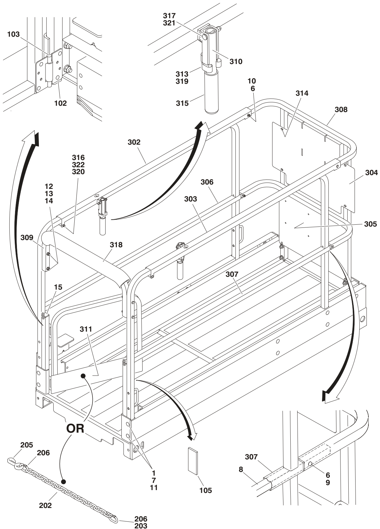
FIGURE 4-3.RAIL (FIXED) INSTALLATION - 1930ES (USA BUILT MACHINES S/N 0200150266 TO S/N 0200152825 & BELGIUM BUILT MACHINES S/N 1200007882 TO S/N 1200008481)
