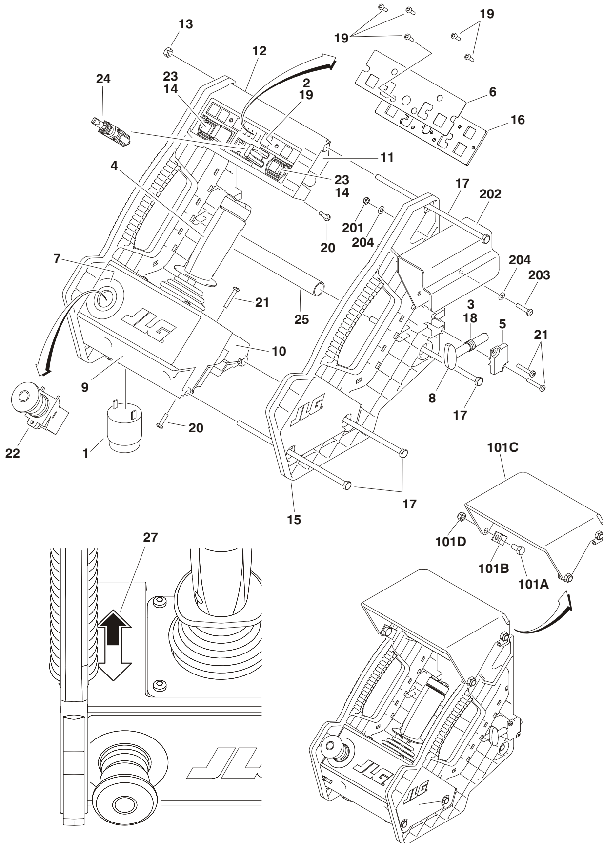
FIGURE 4-9.PLATFORM CONSOLE BOX INSTALLATION
