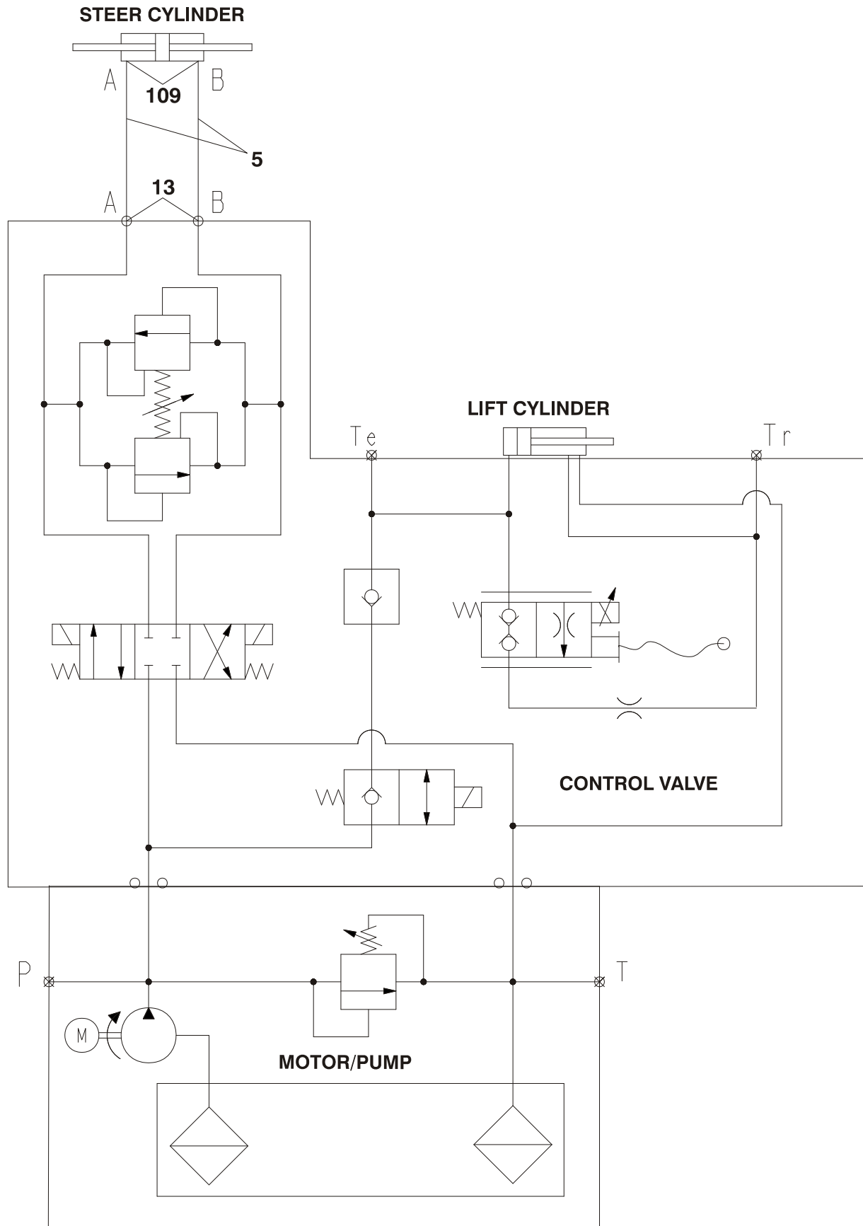
FIGURE 6-1.HYDRAULIC DIAGRAM
