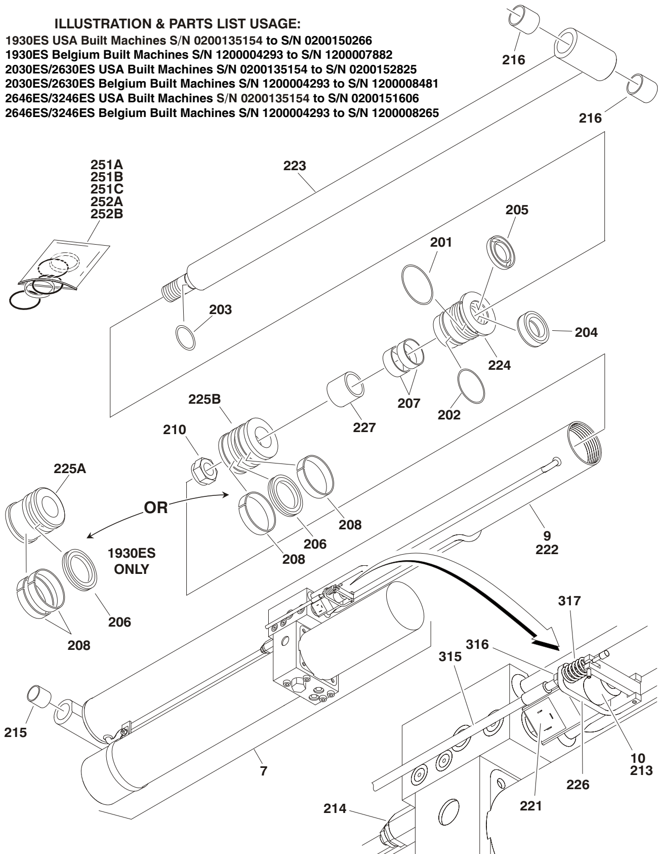
FIGURE 5-1. LIFT CYLINDER ASSEMBLY (FOR MODEL & S/N USAGE SEE TOP OF PARTS LIST)
