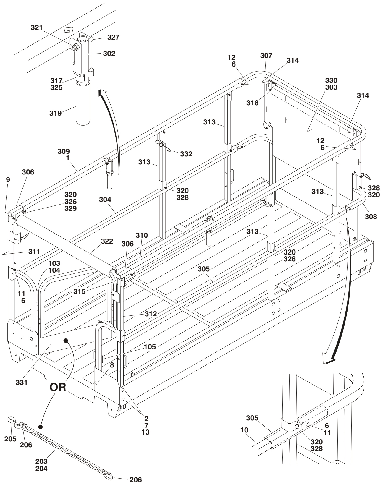
FIGURE 4-8.RAIL INSTALLATION - 2646ES/3246ES (USA BUILT MACHINES S/N 0200151585 TO S/N 0200152825 & BELGIUM BUILT MACHINES S/N 1200008265 TO S/N 1200008481)
