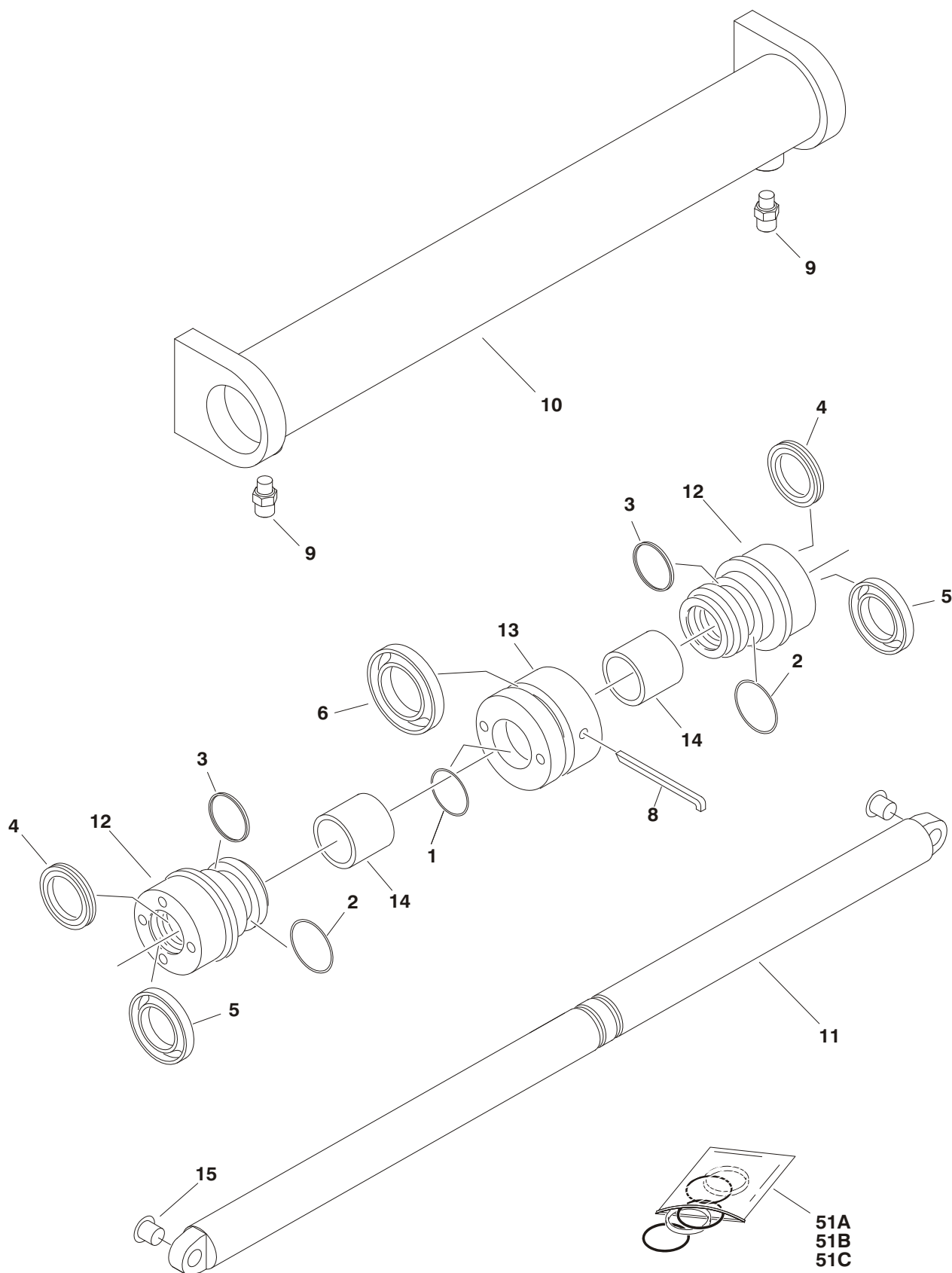
FIGURE 5-3. STEER CYLINDER ASSEMBLY
