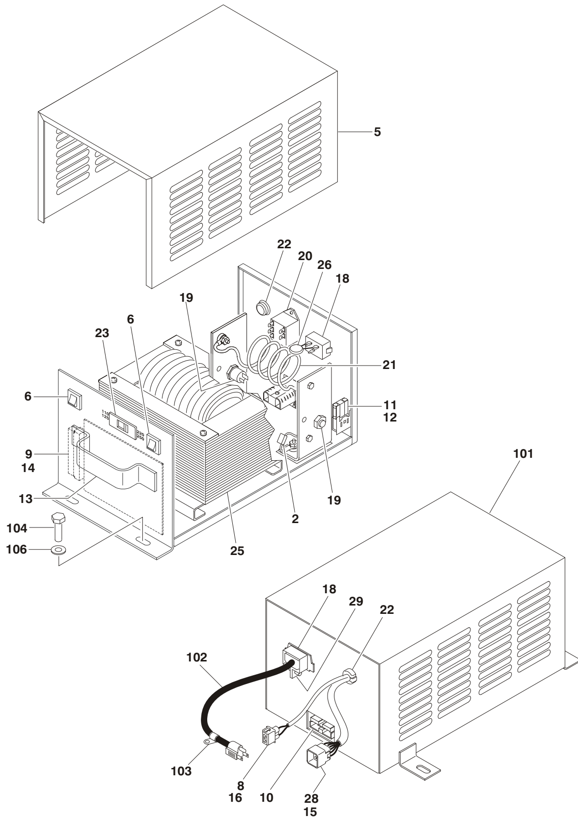
FIGURE 1-7. BATTERY CHARGER ASSEMBLY AND INSTALLATION (MAC CHARGER WITH BREAKERS ON END)
