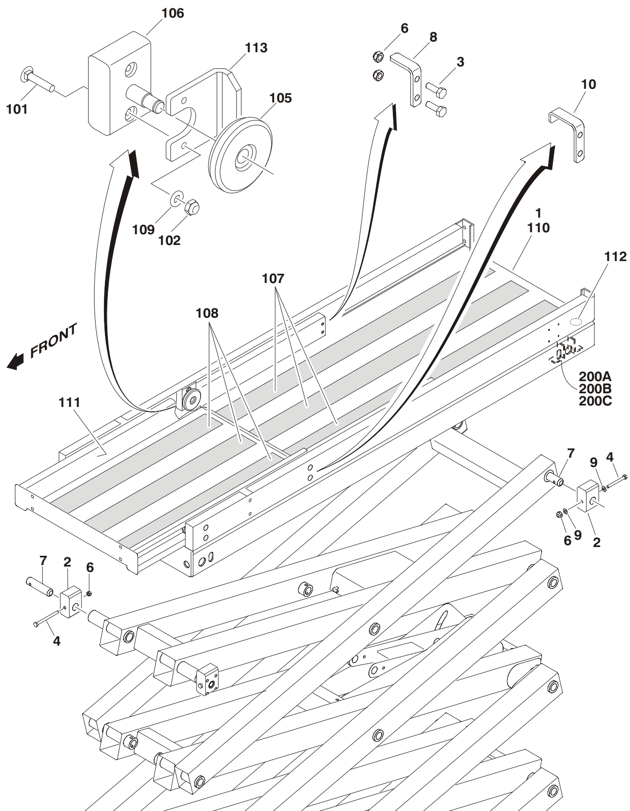
FIGURE 4-1. PLATFORM INSTALLATION
