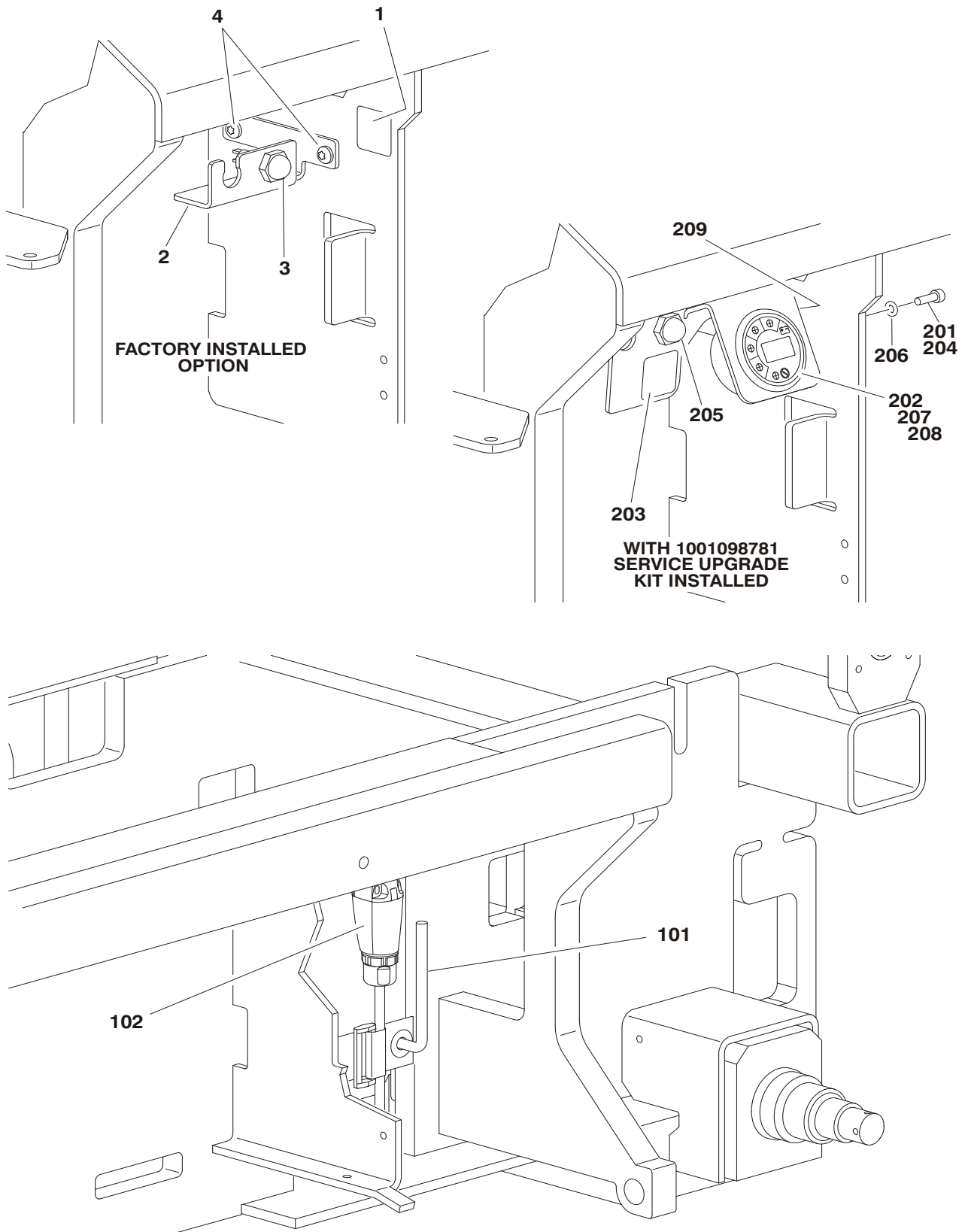
FIGURE 2-3. BRAKE DISCONNECT/RELEASE & MDI (MULTIFUNCTION DIGITAL INDICATOR) GAUGE INSTALLATIONS (OPTIONAL)
