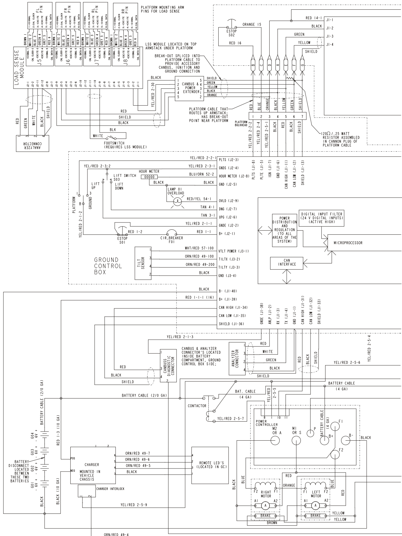
FIGURE 7-1. ELECTRICAL SCHEMATIC (FOR S/N USAGE SEE CHART)
