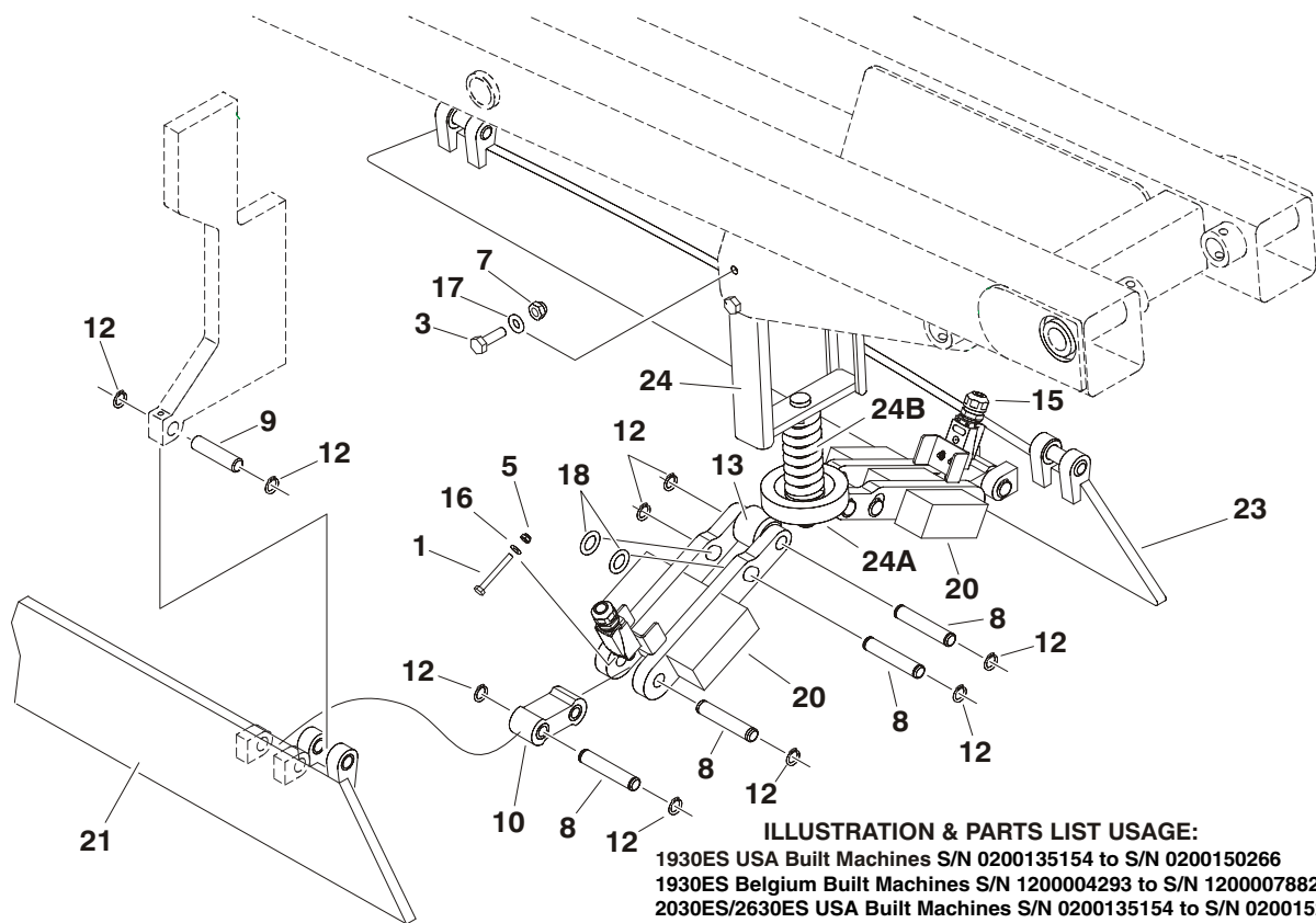
FIGURE 1-5. POTHOLE PROTECTION INSTALLATION (1930ES/2030ES/2630ES)
