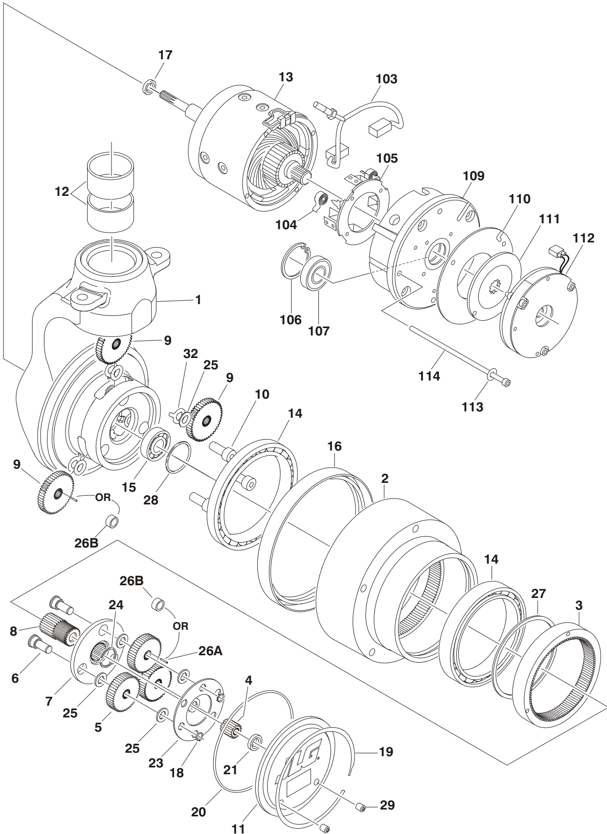
FIGURE 1-3.WHEEL DRIVE ASSEMBLY
