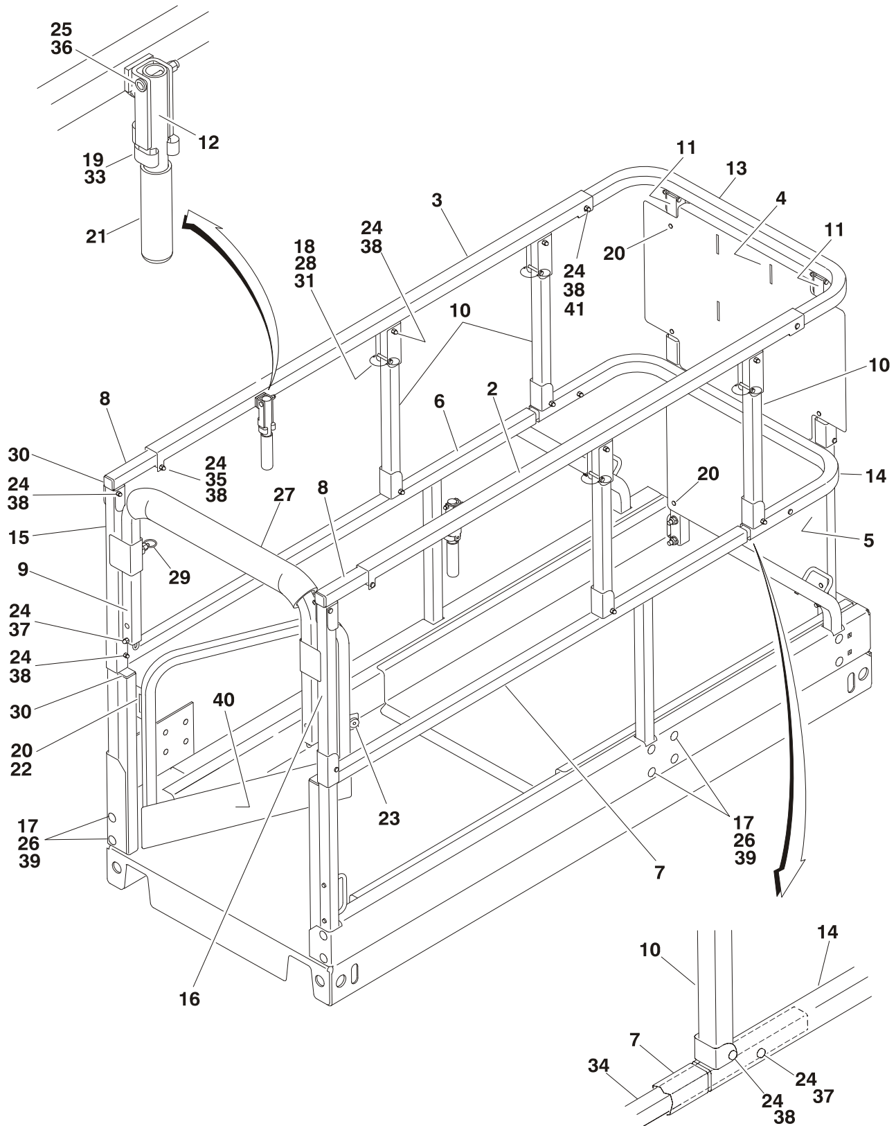
FIGURE 4-4.RAIL (FOLD-DOWN) INSTALLATION - 1930ES (USA BUILT MACHINES S/N 0200135154 TO S/N 0200150266 & BELGIUM BUILT MACHINES S/N 1200004293 TO S/N 1200007882)
